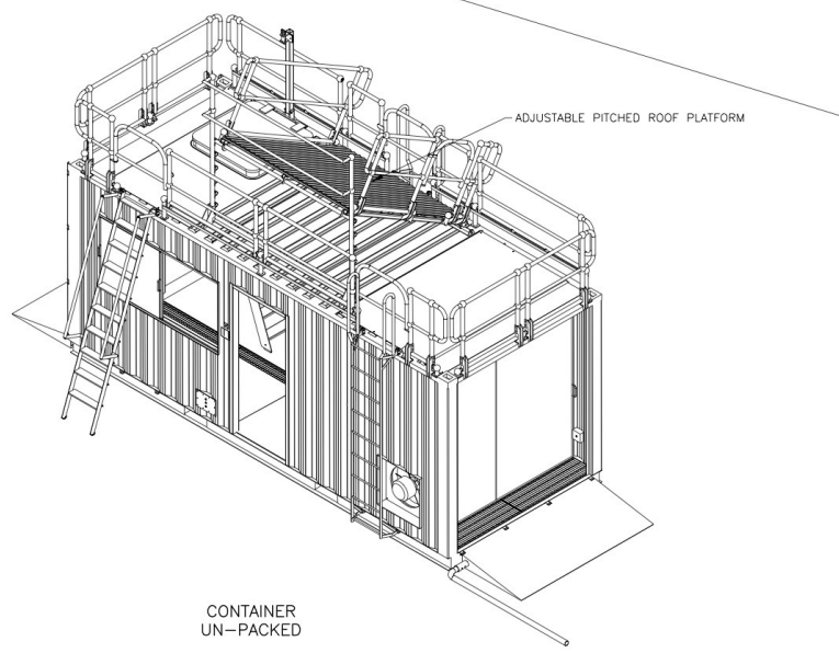
Layout drawing
